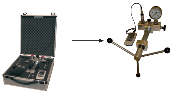
Variant 4: Calibration case with max. 5 pressure sensors and incl. hand spindle pump
