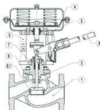
VPA26S— with pneumatic actuator and manual operation
