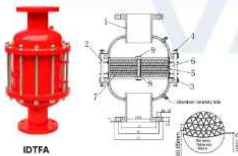
Model : IDTFA (IN LINE DETONATION FLAME ARRESTER)
