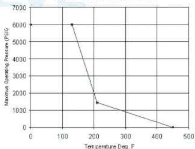
Maximum Operating Pressure - Temperature Data 1/8" to 1" Needle Valve Model VND1
