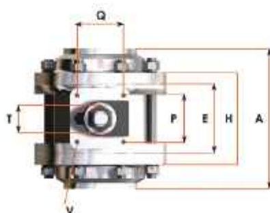
Full Bore DN 50-100 (2" - 4")
