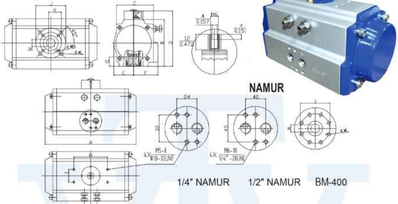
Dimension Table
