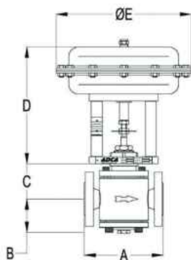
DIMENSIONS - VALVE BODY VPC-32
