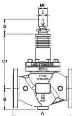
Valve with extended bonnet
