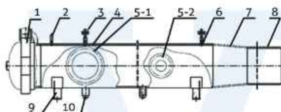
Pig launcher receiver
