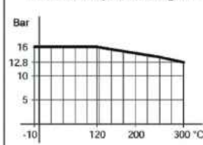
Pressure/Temperature diagram
