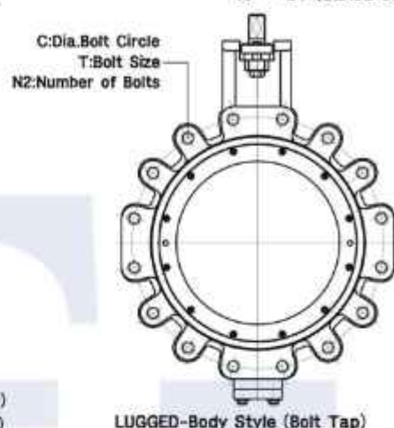
Valve Size : 18" - 24" (CLASS 150) 16" - 24" (CLASS 300)
